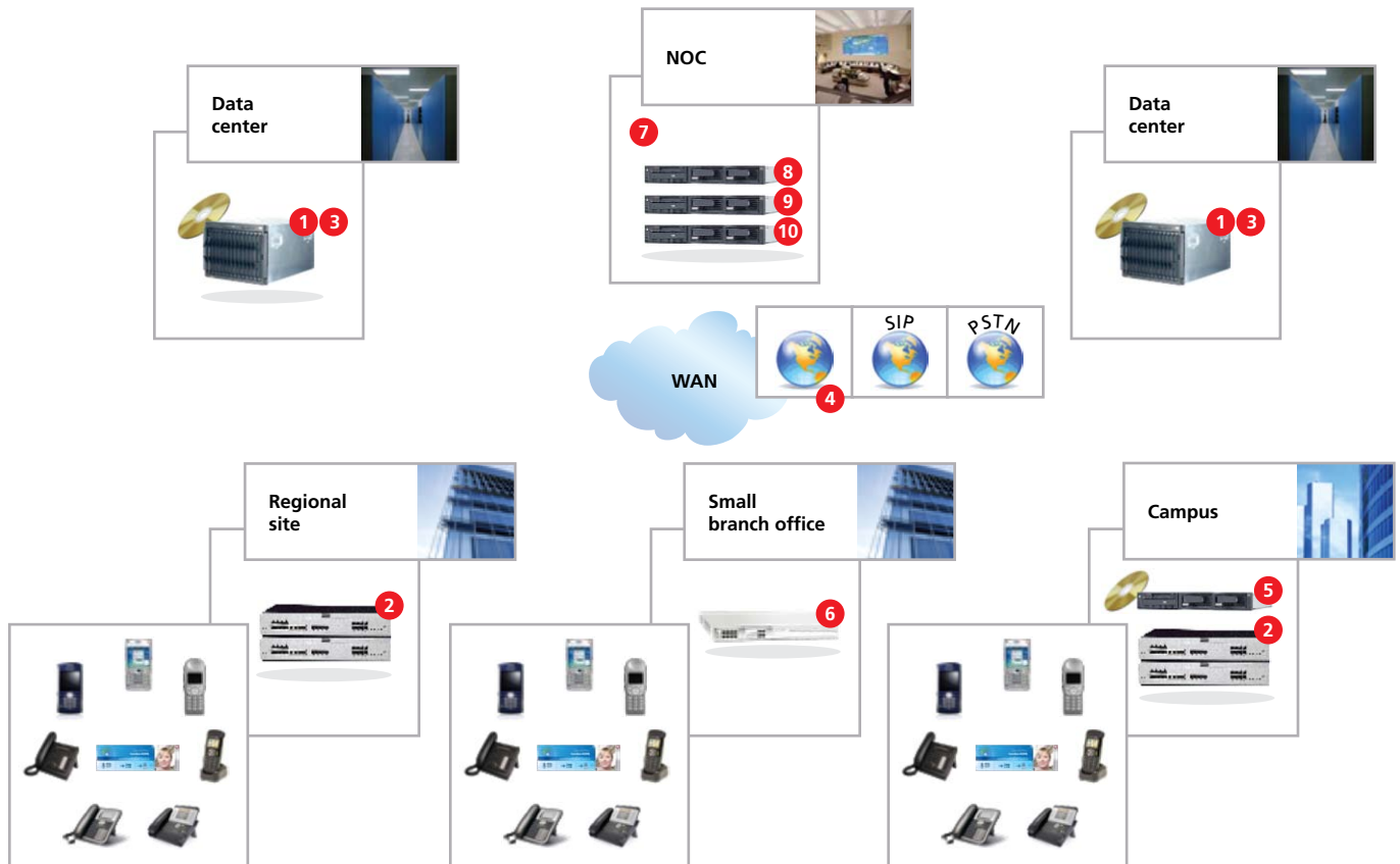
Figure 1. Alcatel-Lucent IP Communications centralized architecture
